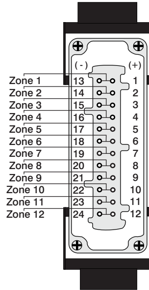
HBE24 Female Insert Dual Latch
