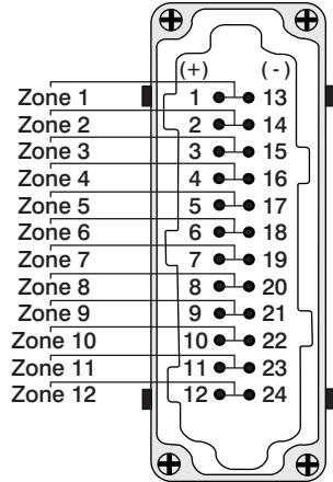
HBE24 Male Insert Dual Latch
