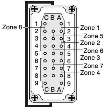
HD25 Female Insert Single Latch
