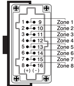
HBE16 Male Insert Single Latch
