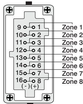
HBE16 Female Insert Single Latch
