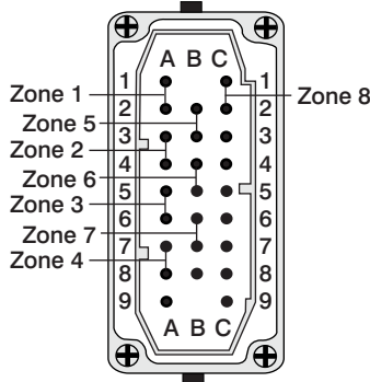
HD25 Male Insert Single Latch
