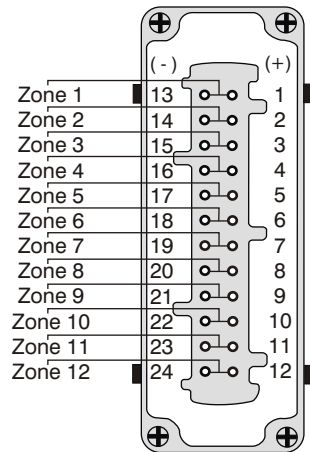
Female Insert Dual Latch
