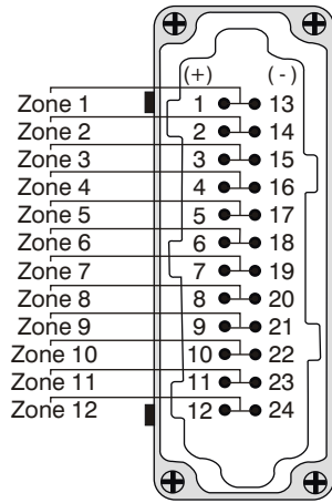
Male Insert Dual Latch
