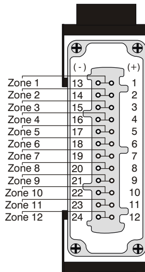
Female Insert Dual Latch
